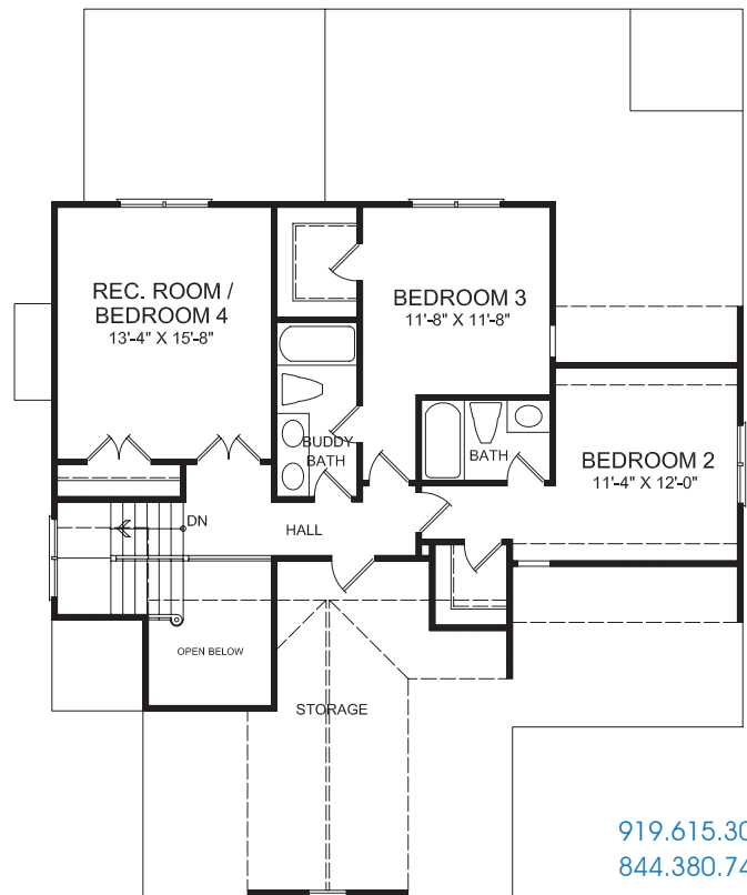
SECOND FLOOR
